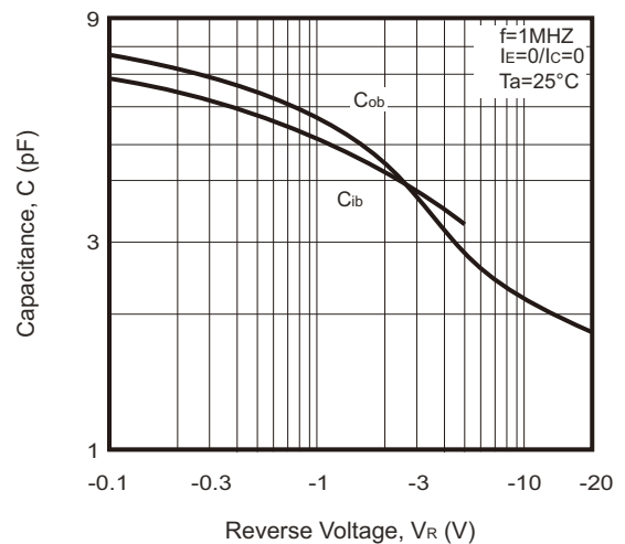
Fig.6 - C_{ob}/C_{ib} - V_{CB}/V_{EB}
